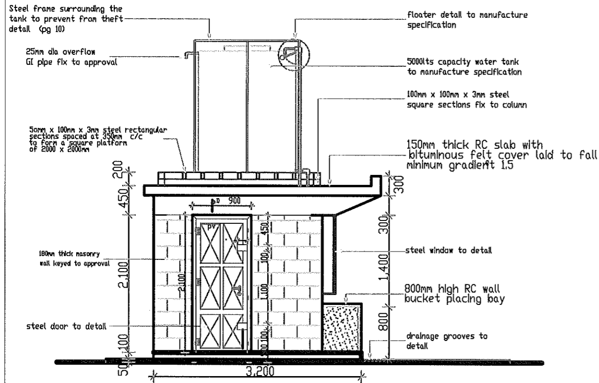
SIDE ELEVATION
