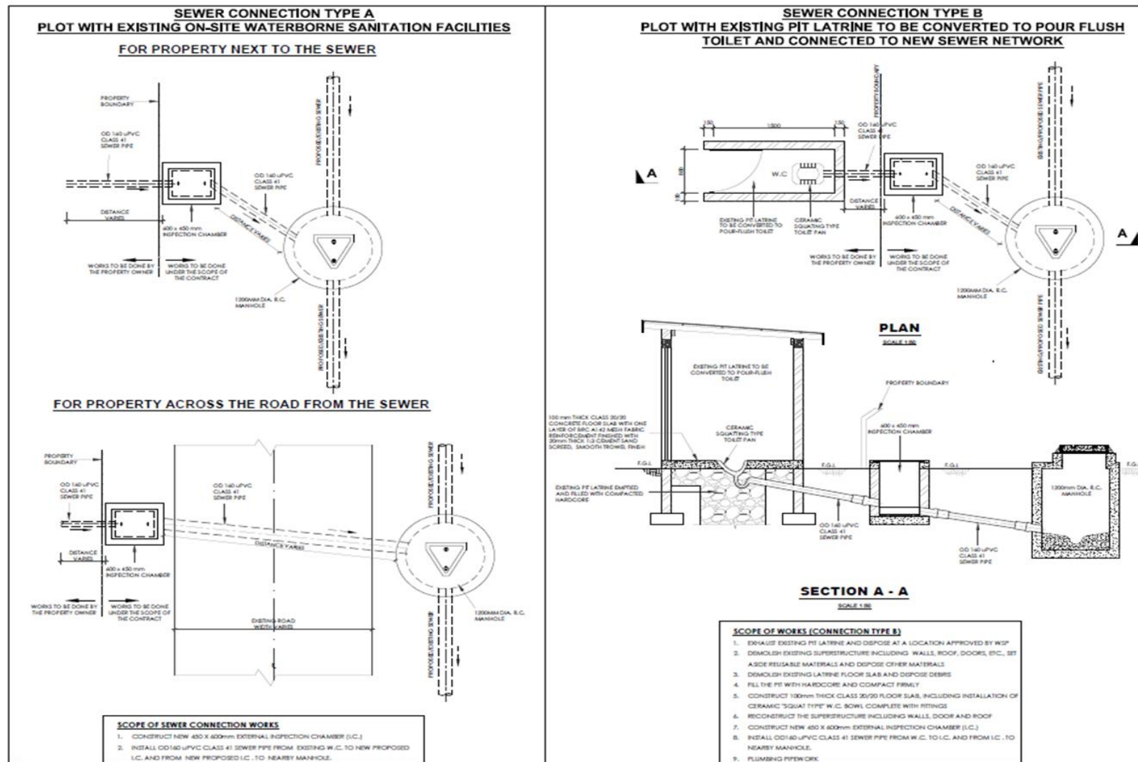
Figure 3: Typical Sewerage connection
