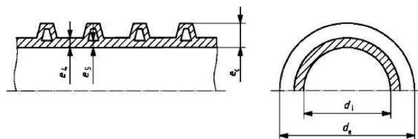
Figure 1 – corrugation diagram
